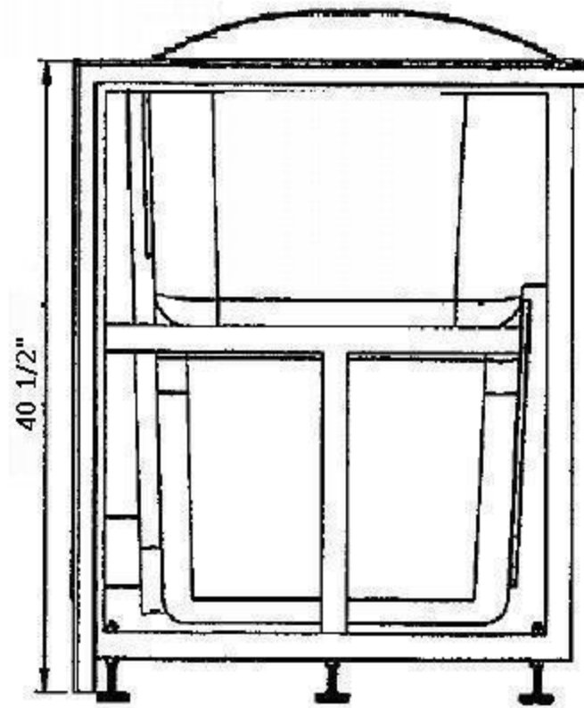
RIGHT VIEW
